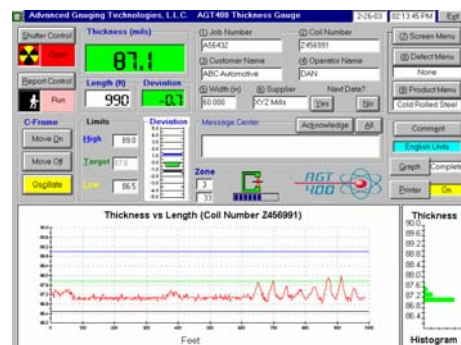
AGT400 Thickness Gauge & S.P.C. Reporting System
